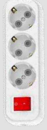
516-010200-302 Child Protected 3Gang Earthed Cordless With Rocker Switch 3'Lü Çocuk Korumalı ATGP KL
